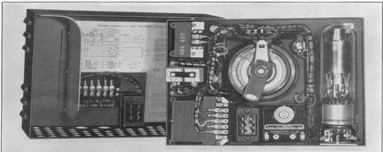
Figure 3. Interior view of the Variac Speed Control.
