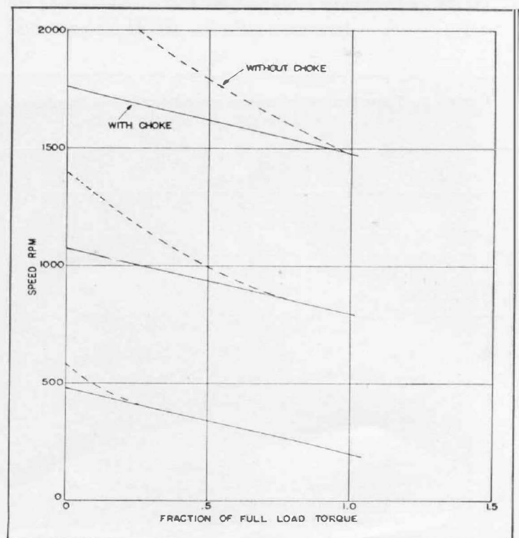
Figure 5. Regulation curves at various speeds for the Type 1700-AH Variac Speed Control. Dotted lines show performance of a similar system without choke.
