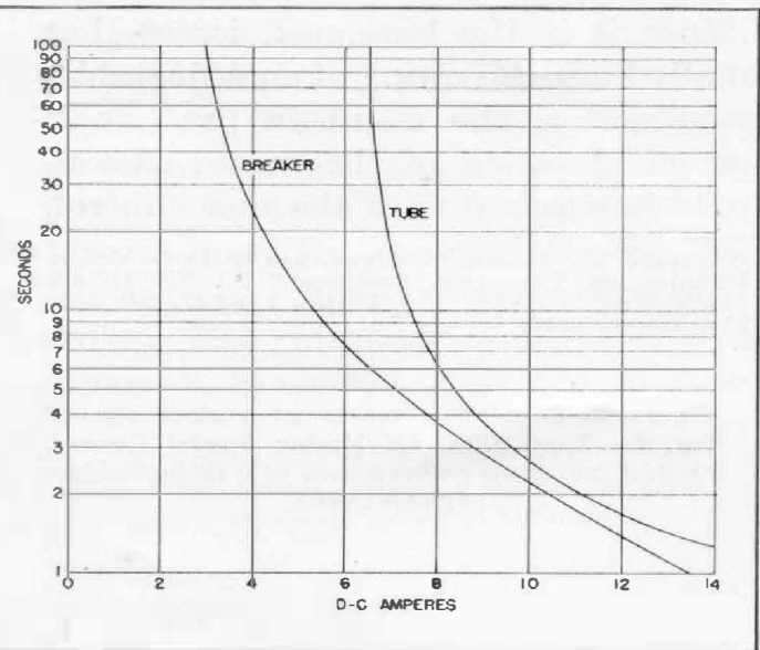
Figure 7. Overload characteristic of rectifier tube and delay characteristic of circuit breaker.
