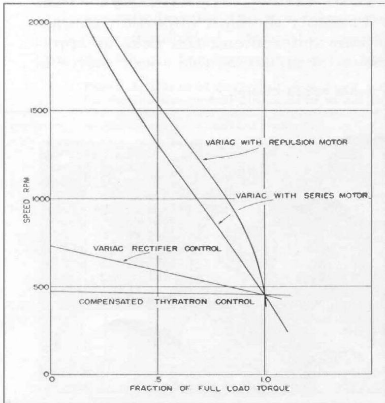
Figure 4. Comparison of the performance of various types of control systems adjusted for one-quarter maximum speed at full load.
