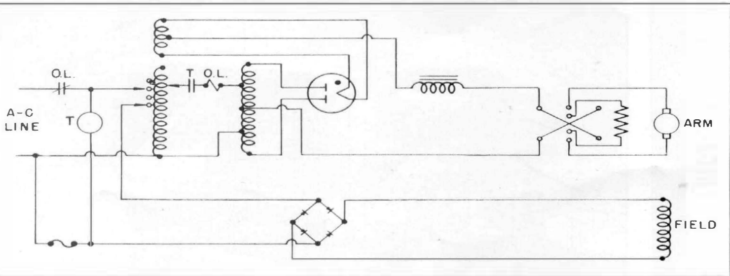
Figure 2. Circuit of the speed control unit. Industrial, rather than radio, symbols have been used for those elements that are peculiar to industrial equipment. Hence, the symbols T, T refer to the timing clock and its associated switch, and O.L. refers to the overload breaker.
