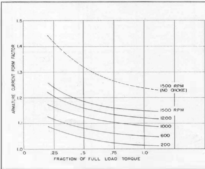
Figure 6. Form factor of armature current as a function of load at various speeds.
